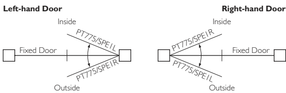
Extended Strike Plate to suit 775 Series Mortice Lock Left-handed. (Suits left-hand opening in: right-hand opening out) PT775/SPEIL SSS
